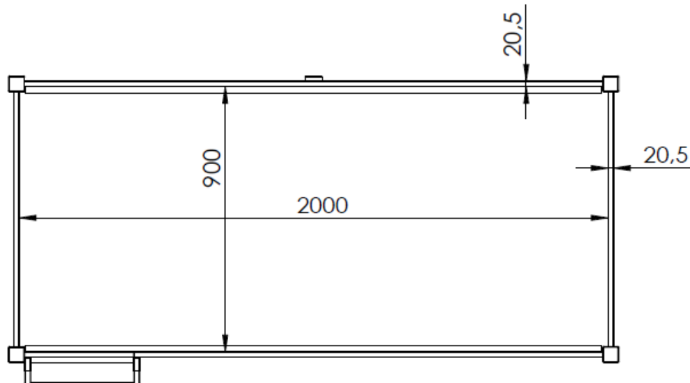
MATTRESS 900x2000 mm
