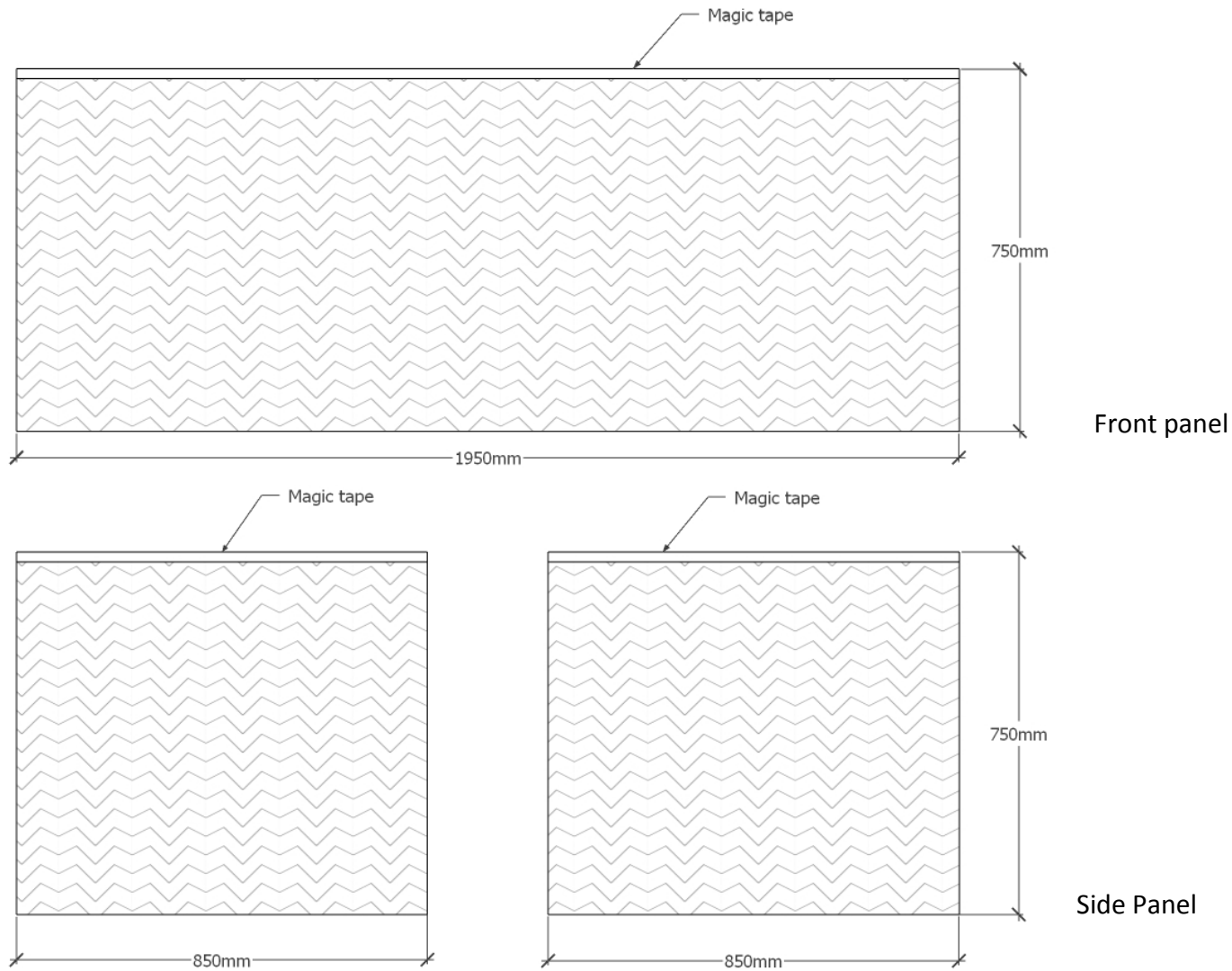
Bed Tent Mid sleeper : 1 Front-panel , 2 Side-panels
