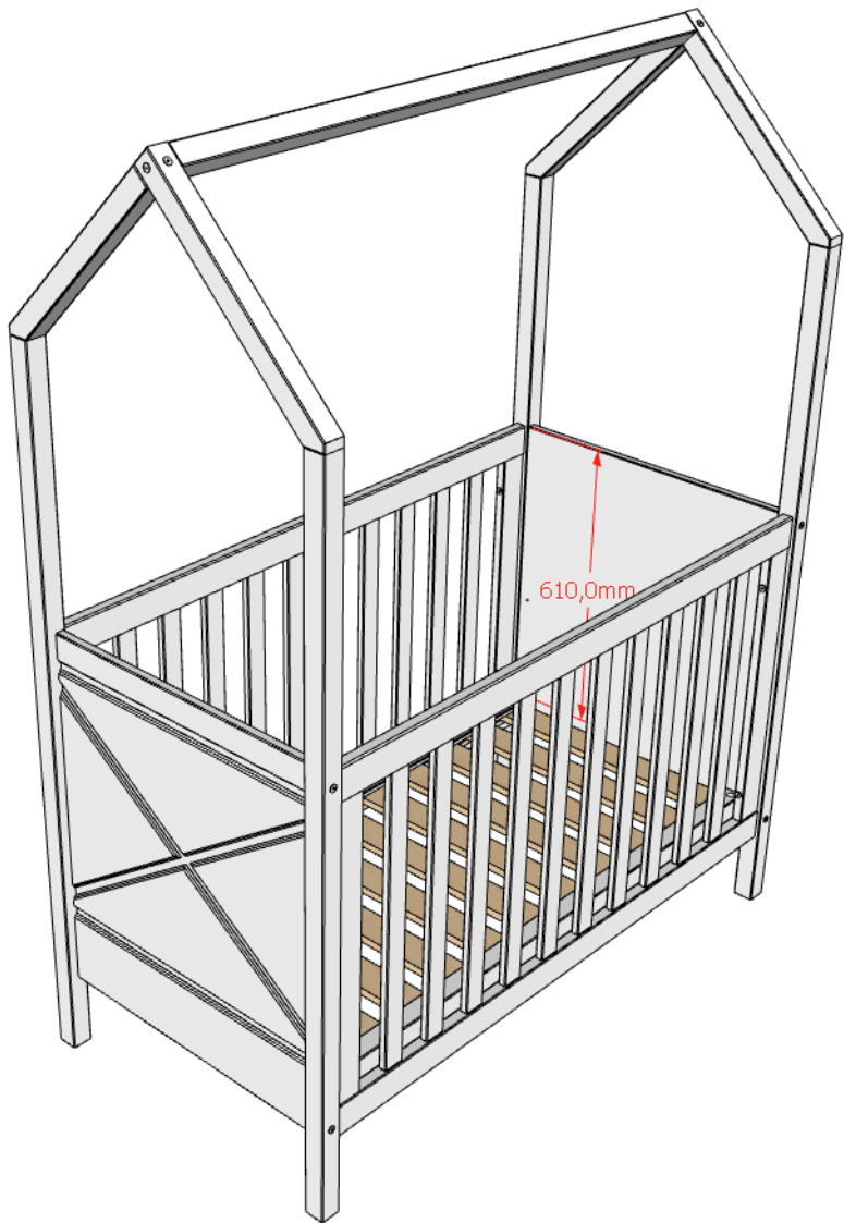
BABYBED TESTING ACCORDING EN 716-2:2017 CLASIFICACION ACCORDING EN 716-1:2017+AC:2019
