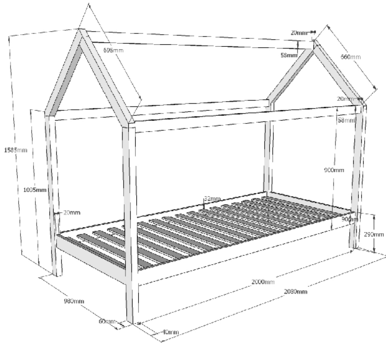
L:2080mm H:1585mm D:980mm innersize 900x2000mm 17 Slats 60x12mm plywood
