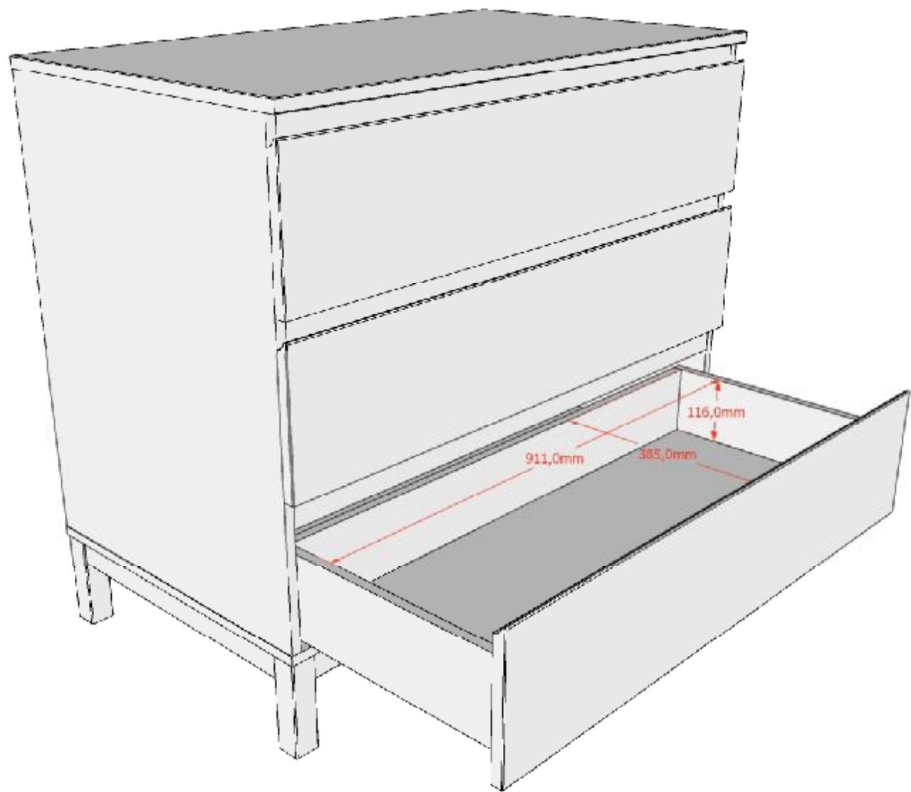
DRAWERS WITH SOFTCLOSING GLIDERS
