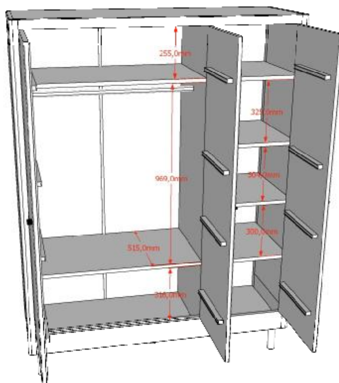
DOORS WITH SOFCLOSE HINGES
